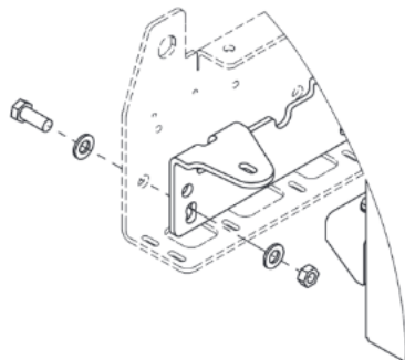
Placement of mounting brackets 6340557 1300K/1730K
