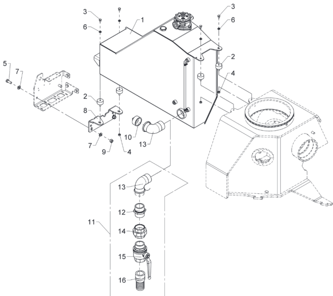
Placement of mounting brackets 6340557 1300K/1730K
