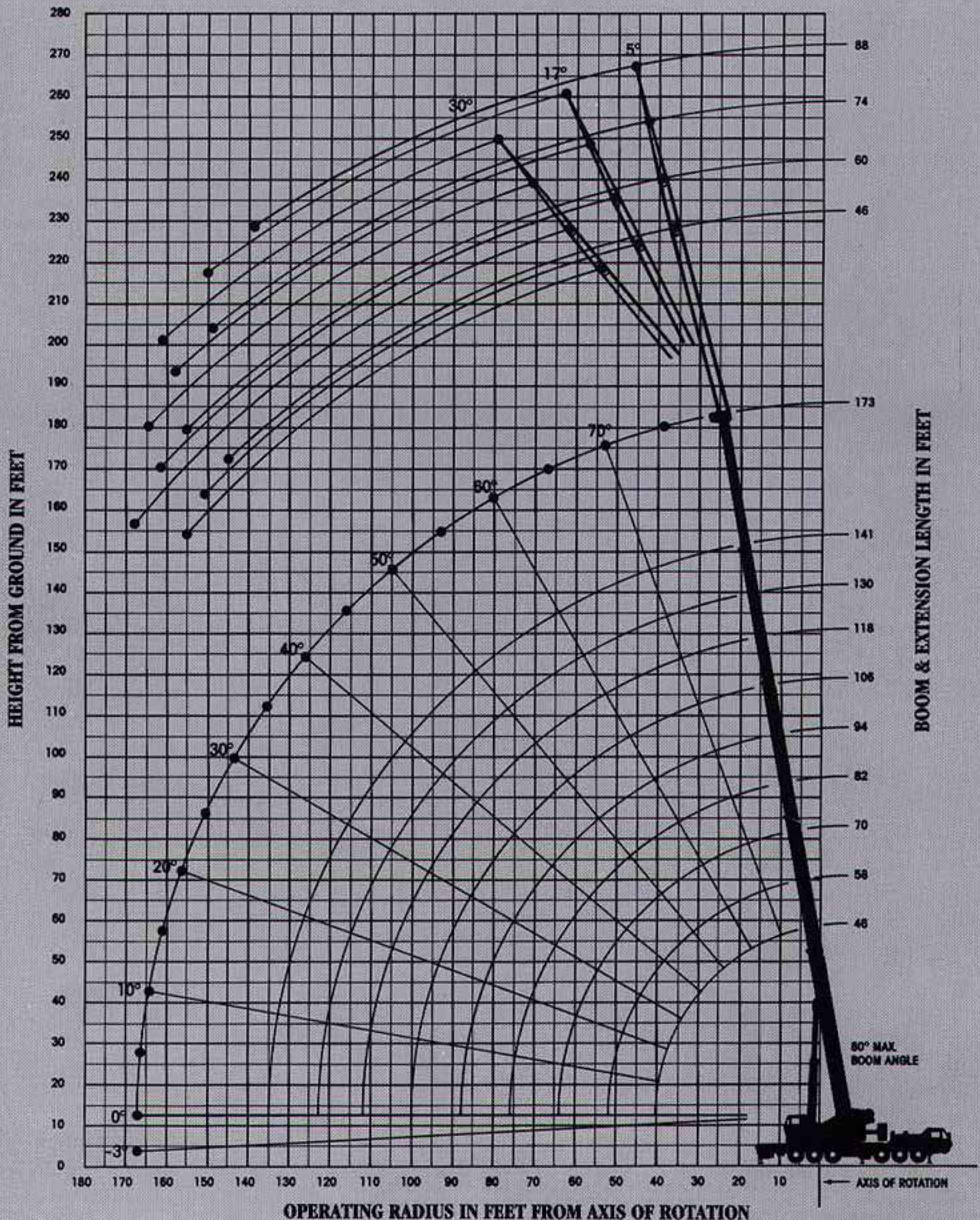
WORKING RANGE DIAGRAM (BOOM DEFLECTION NOT SHOWN)
