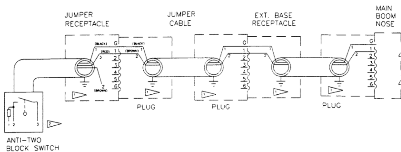
TELE. EXTENSION WIRING DIAGRAM
