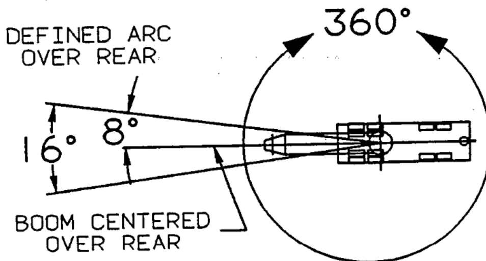
LIFTING AREA DIAGRAM ON TIRES
